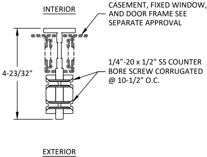
C 2 CROSS SECTION FT 1201042TF-14
