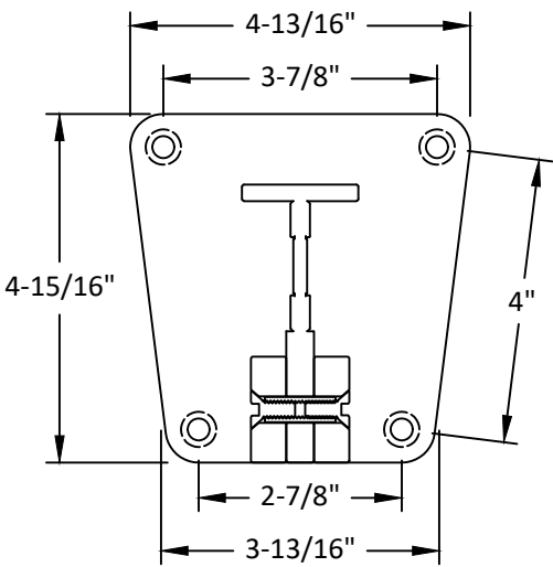
MULLION PLATE DETAIL 1/4" THICK, FT 1001042TF-14
