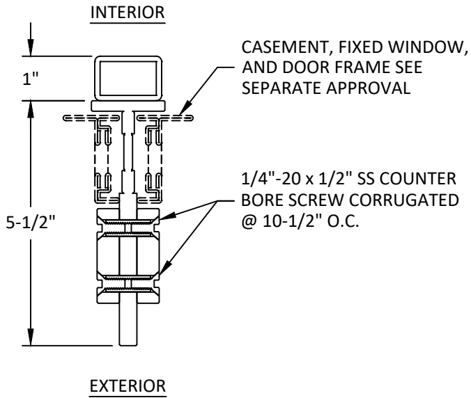
E 2 CROSS SECTION FT 1401042TF-14 W/ 1" x 1.5" x 1/8" TUBE
