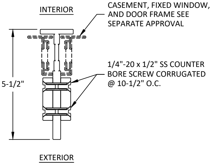
D 2 CROSS SECTION FT 1401042TF-14
